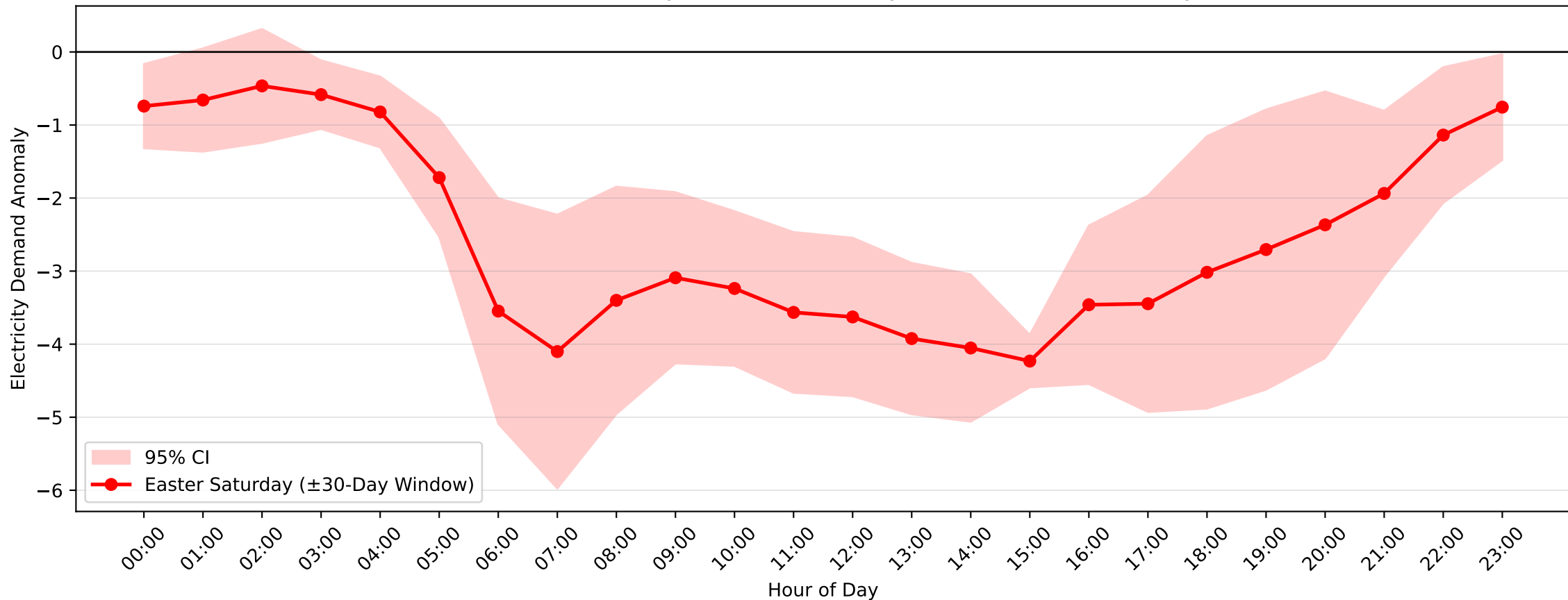
Kirrawee Demand Anomaly: Easter Saturday (2004-2017, \pm 30 -Day Window)
